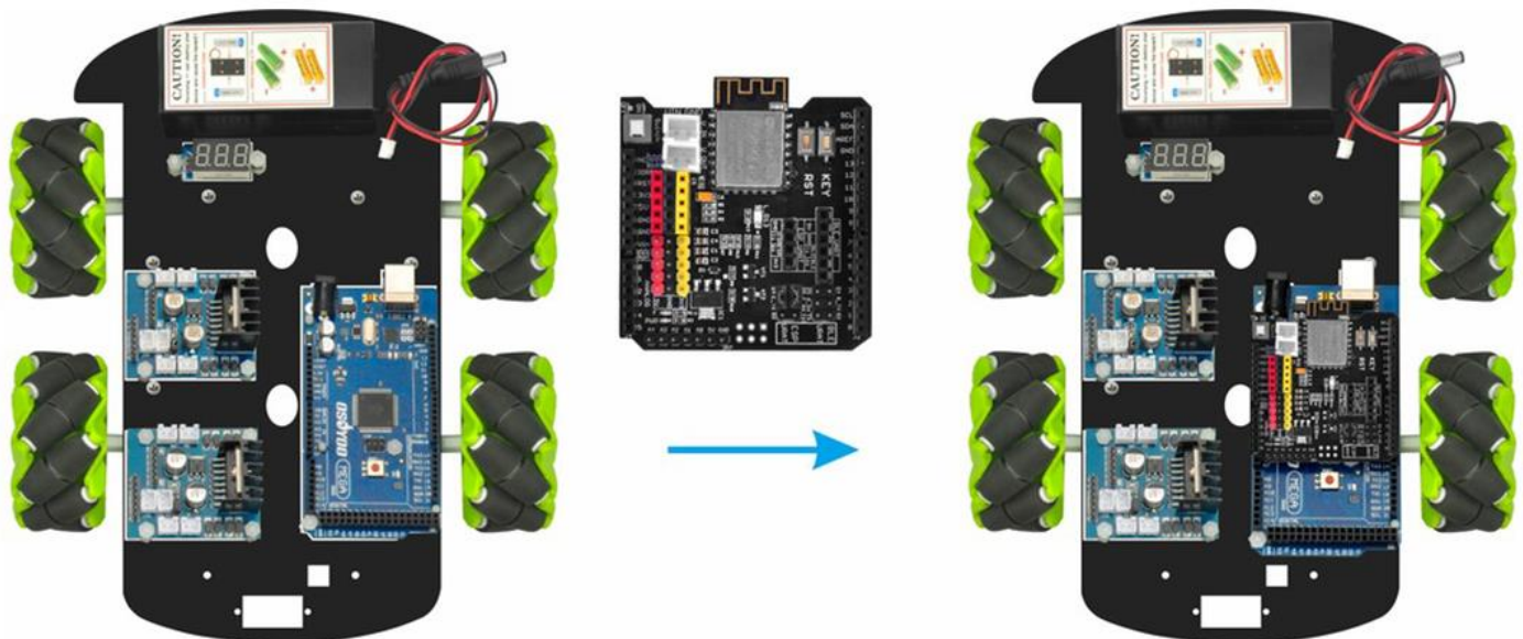
Step7: Insert OSOY00 Uart WIFI shield onto your mega2560 board.
